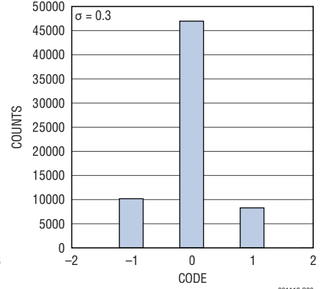
DC Histogram for 64k Samples
